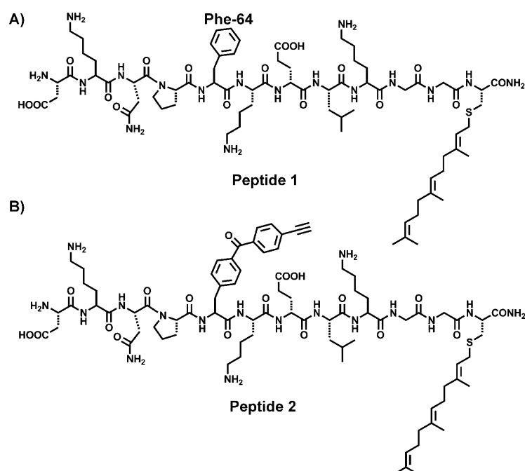
Scheme 1. Peptide 1: native Gt \gamma (60-71)far peptide derived from the transducin Gt \gamma subunit (60DKNPFKELKGGC 71 -farnesyl). Peptide 2: photoactivable Phe-64 p -ethynylbenzoyl-modified peptide 1.
